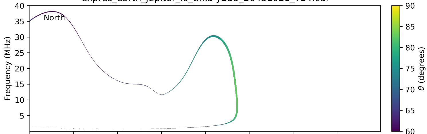
expres_earth_jupiter_io_txka-y235_20431021_v14.cdf
