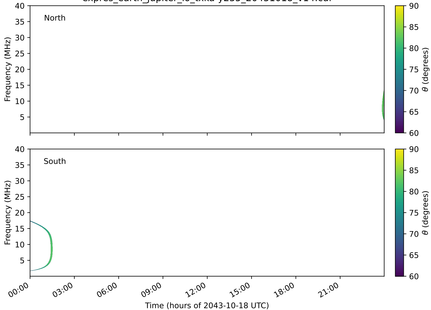
expres_earth_jupiter_io_txka-y235_20431018_v14.cdf
