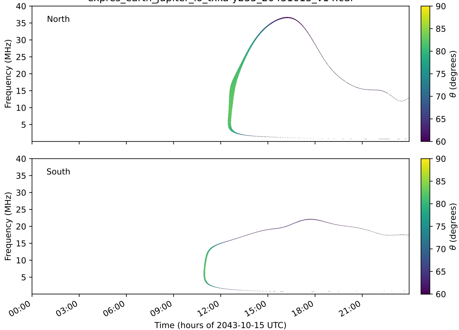
expres_earth_jupiter_io_txka-y235_20431015_v14.cdf
