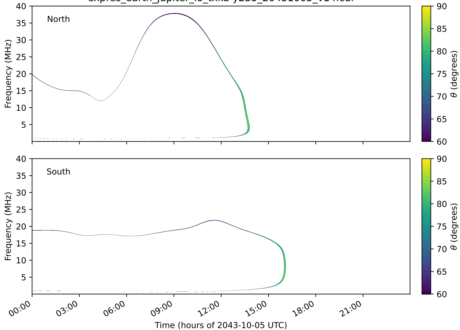
expres_earth_jupiter_io_txka-y235_20431005_v14.cdf
