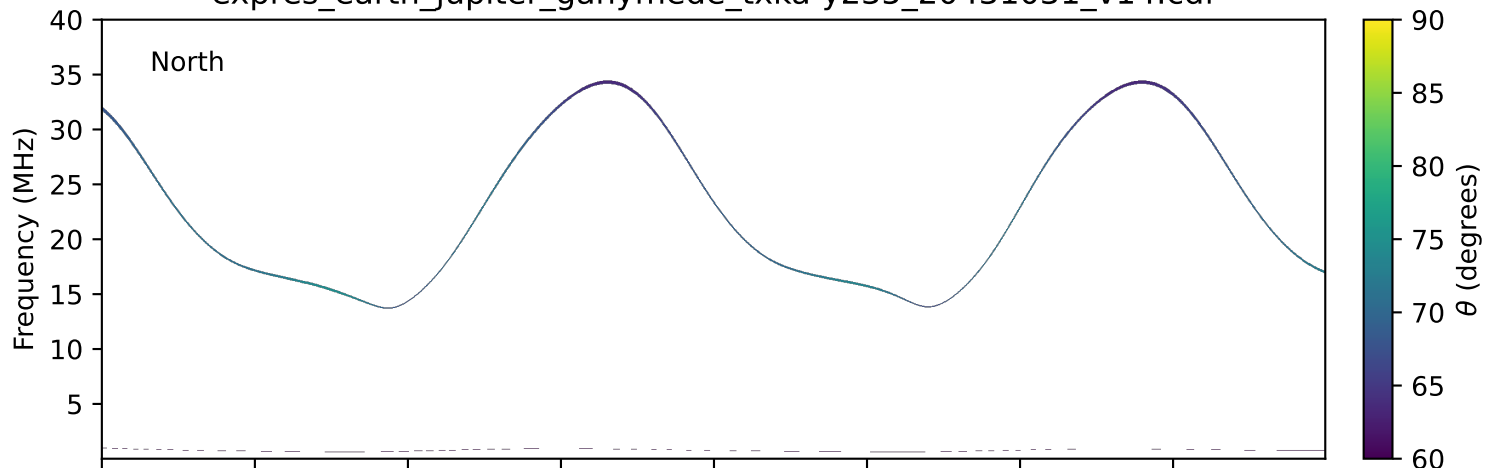
expres_earth_jupiter_ganymede_txka-y235_20431031_v14.cdf
