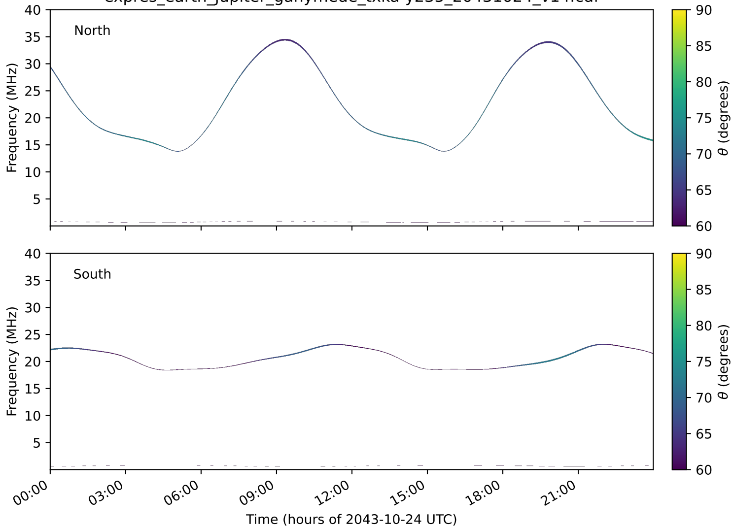
expres_earth_jupiter_ganymede_txka-y235_20431024_v14.cdf
