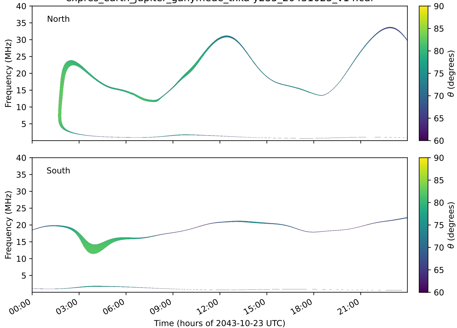
expres_earth_jupiter_ganymede_txka-y235_20431023_v14.cdf
