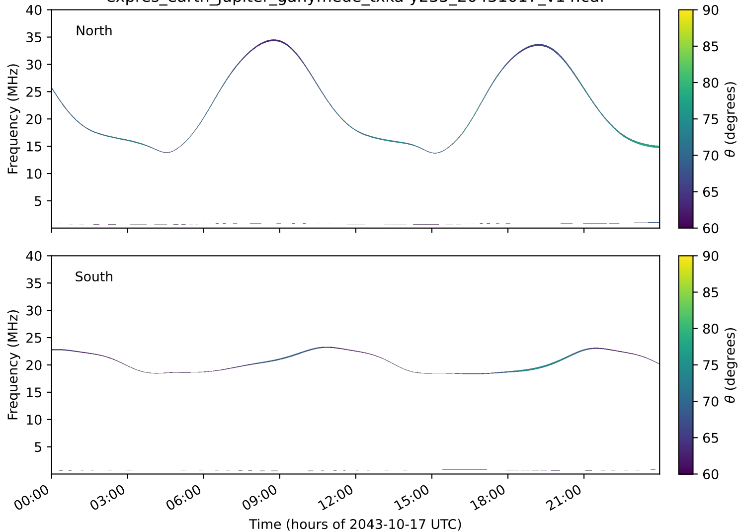
expres_earth_jupiter_ganymede_txka-y235_20431017_v14.cdf
