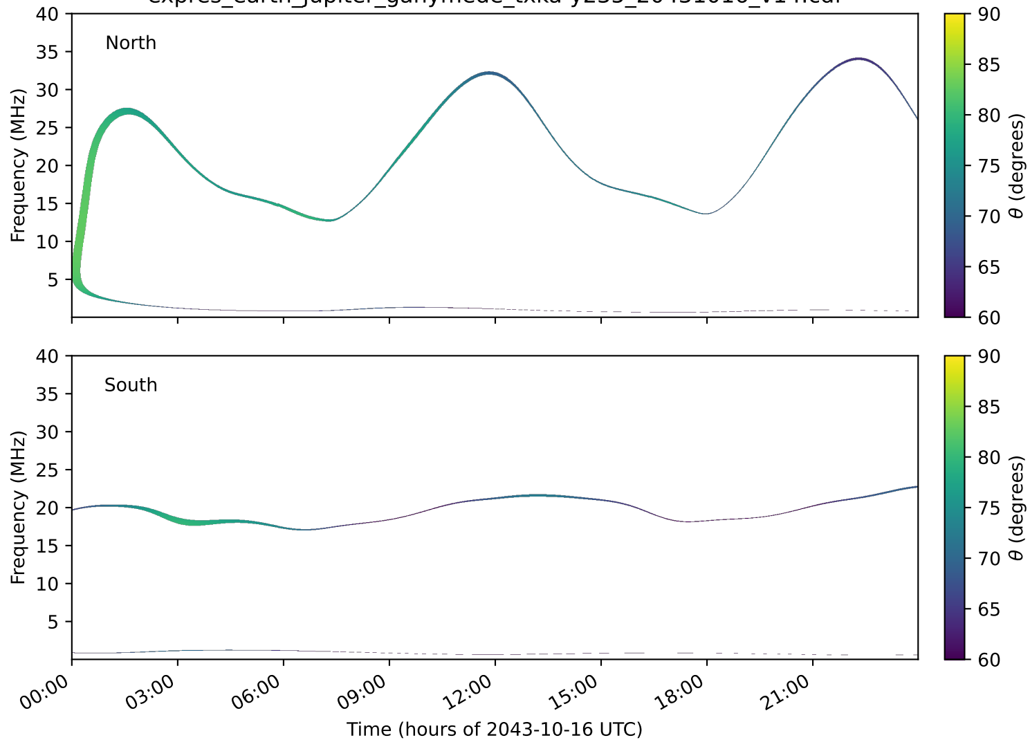
expres_earth_jupiter_ganymede_txka-y235_20431016_v14.cdf
