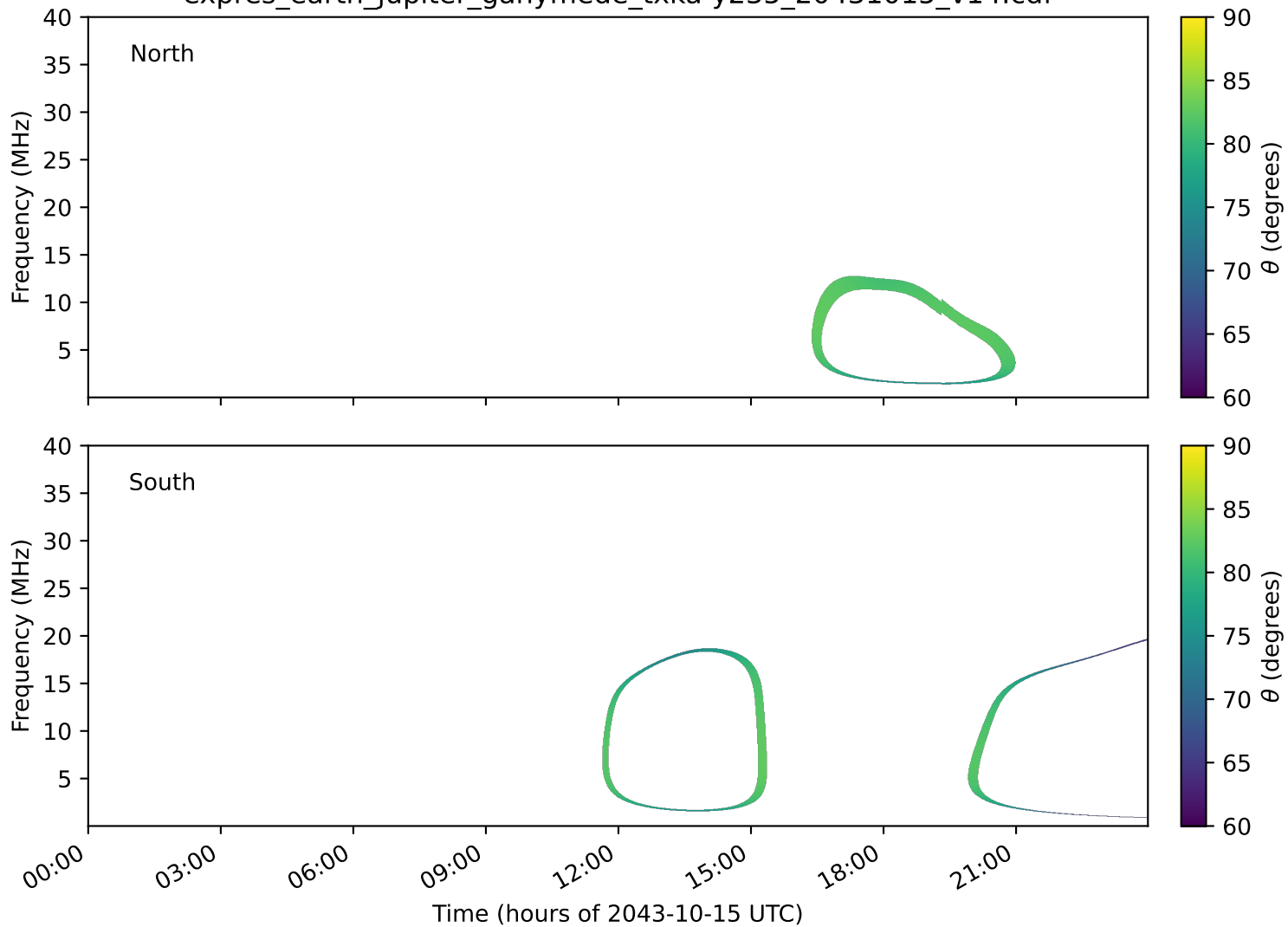
expres_earth_jupiter_ganymede_txka-y235_20431015_v14.cdf
