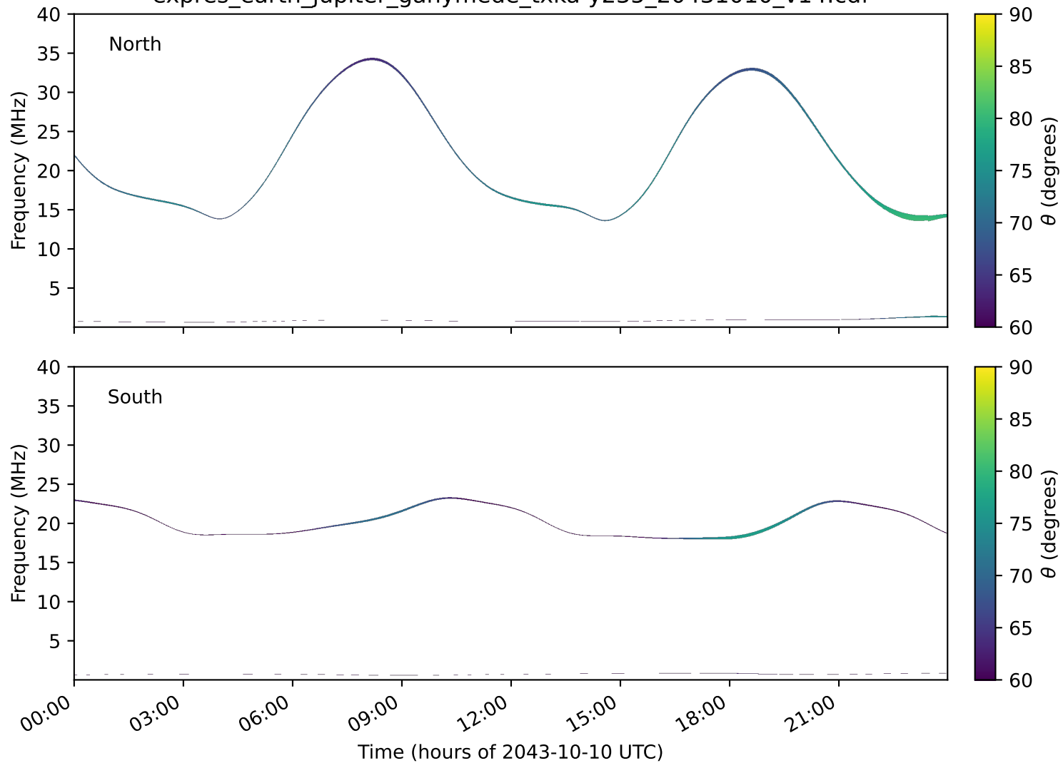
expres_earth_jupiter_ganymede_txka-y235_20431010_v14.cdf
