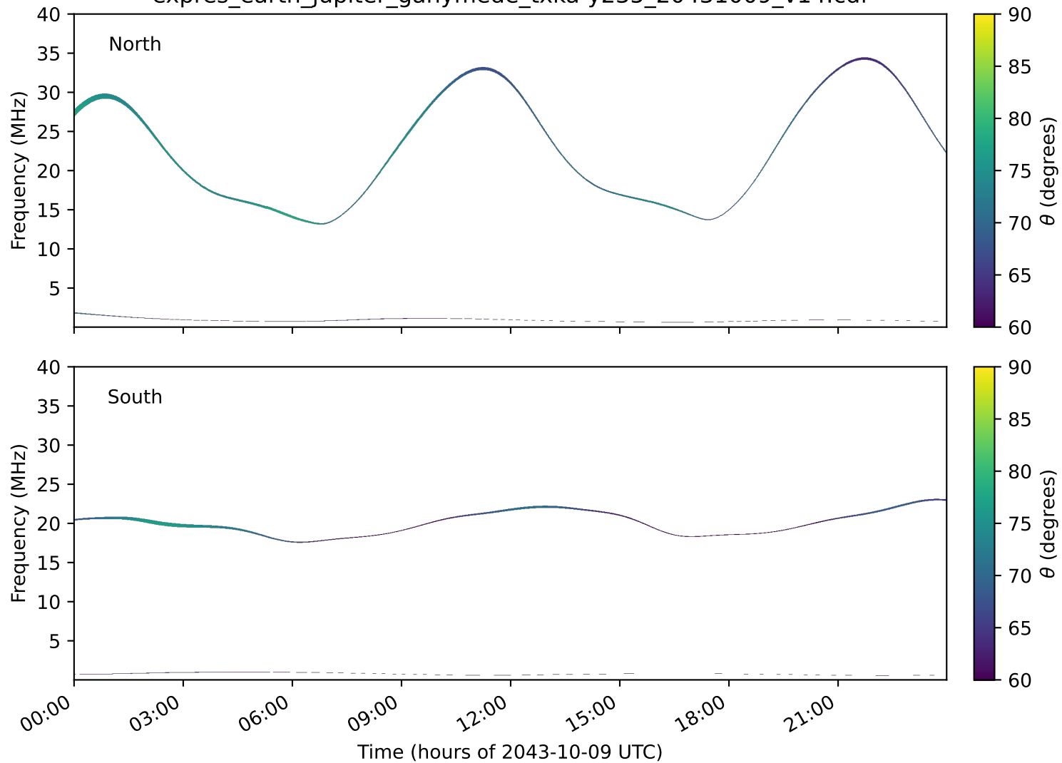
expres_earth_jupiter_ganymede_txka-y235_20431009_v14.cdf
