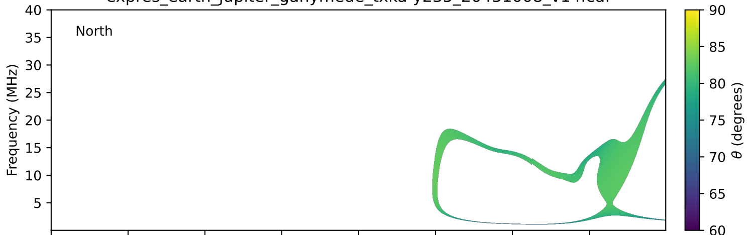
expres_earth_jupiter_ganymede_txka-y235_20431008_v14.cdf
