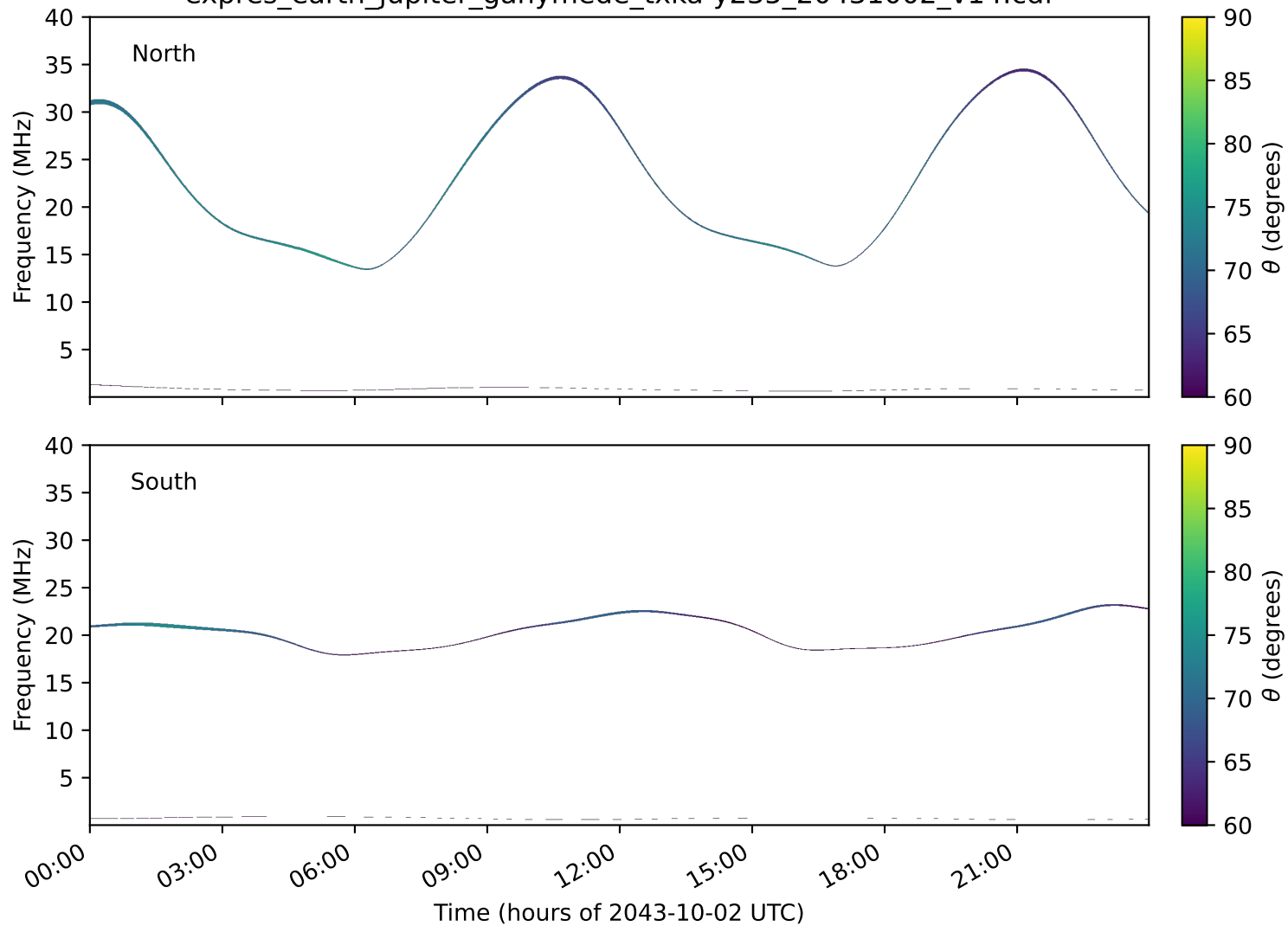
expres_earth_jupiter_ganymede_txka-y235_20431002_v14.cdf
