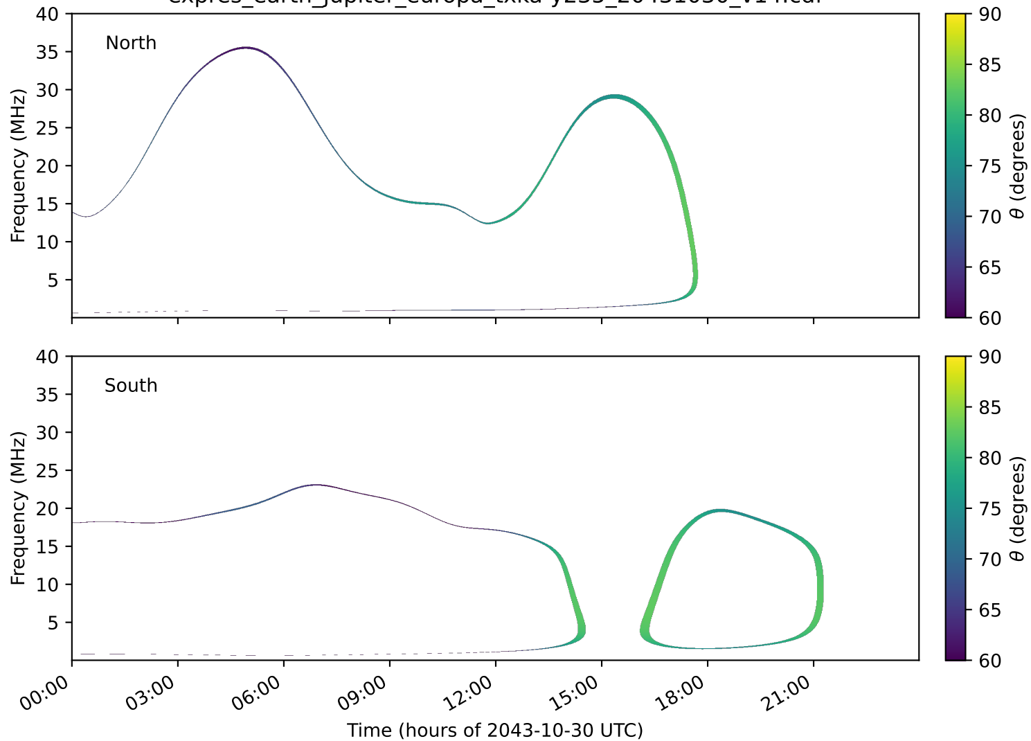
expres_earth_jupiter_europa_txka-y235_20431030_v14.cdf
