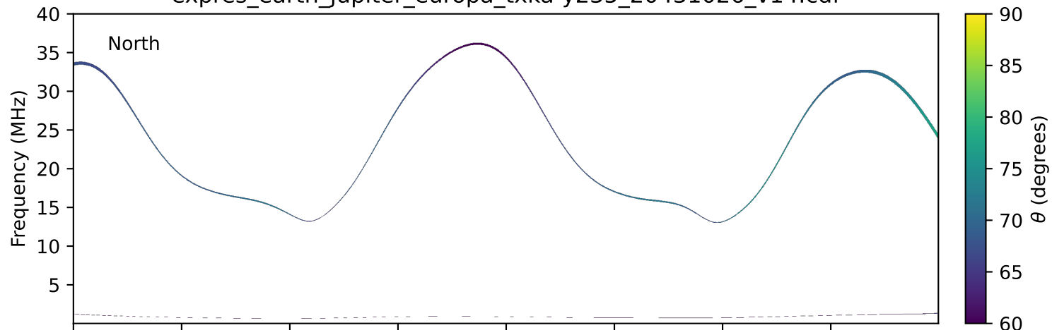
expres_earth_jupiter_europa_txka-y235_20431026_v14.cdf
