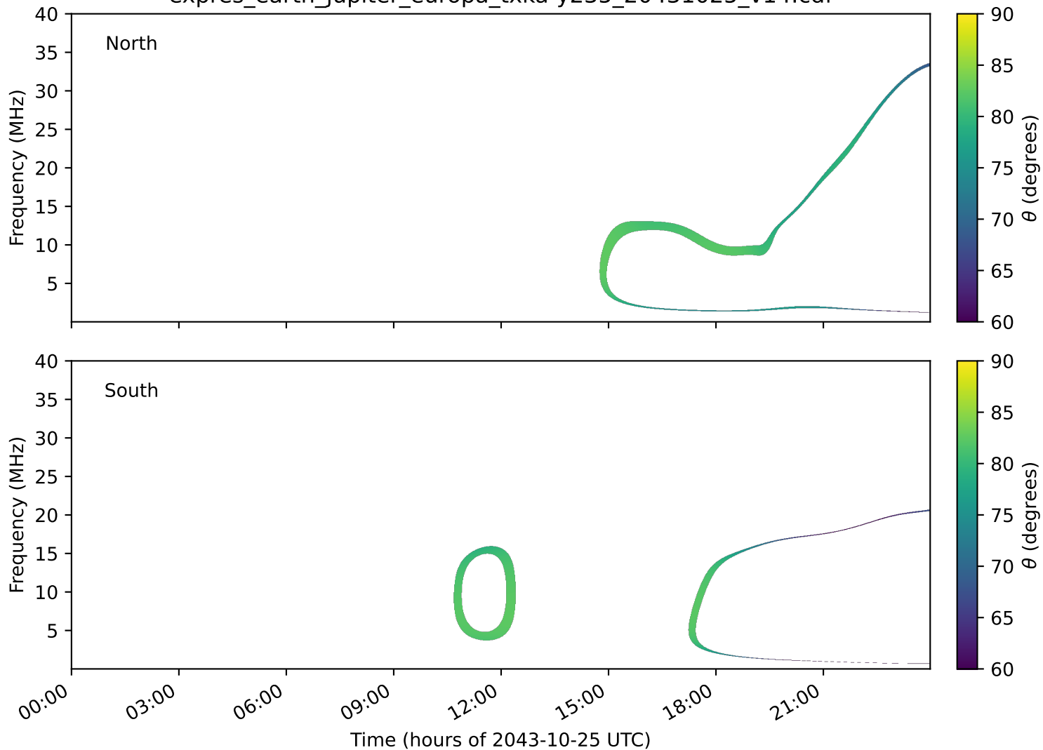
expres_earth_jupiter_europa_txka-y235_20431025_v14.cdf
