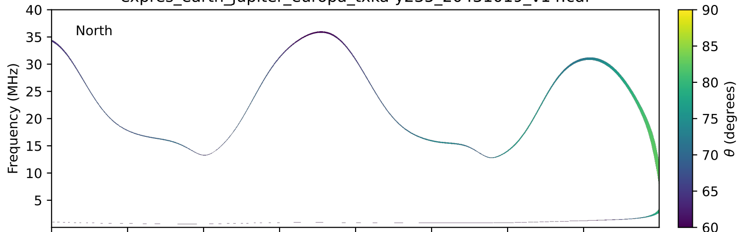
expres_earth_jupiter_europa_txka-y235_20431019_v14.cdf
