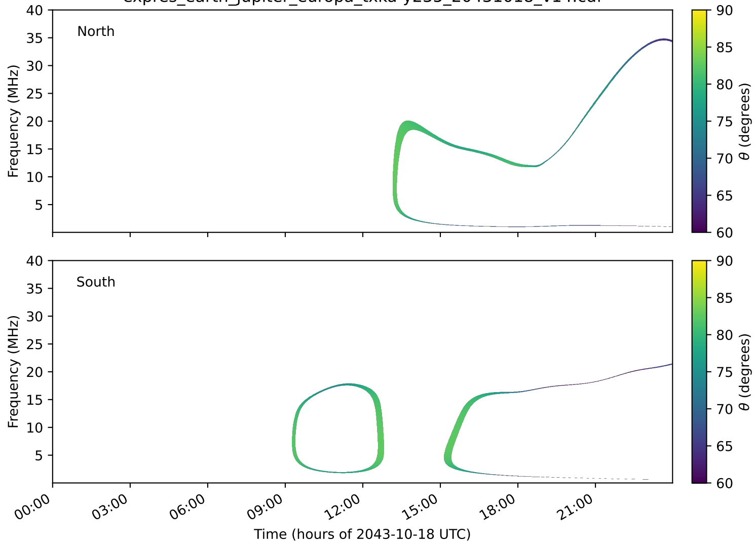
expres_earth_jupiter_europa_txka-y235_20431018_v14.cdf
