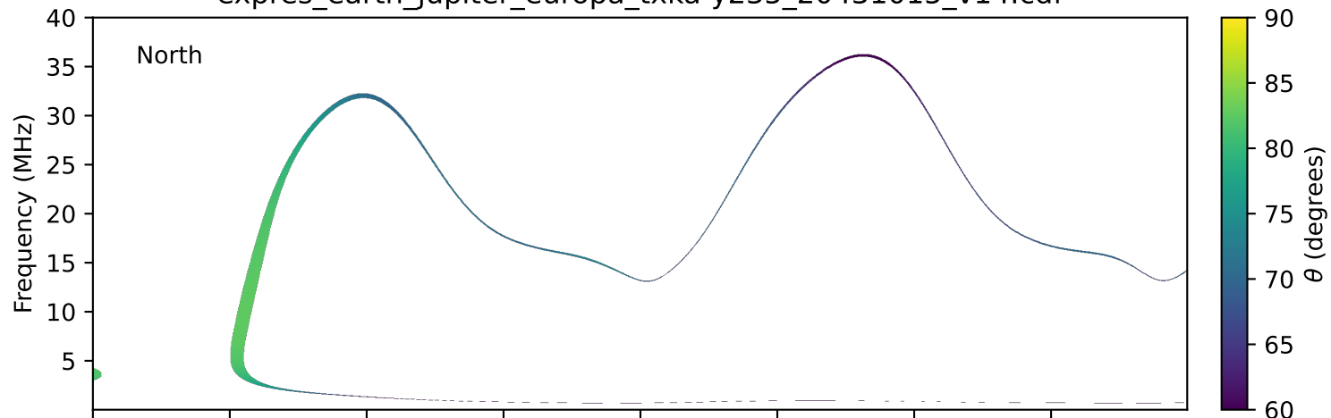
expres_earth_jupiter_europa_txka-y235_20431015_v14.cdf
