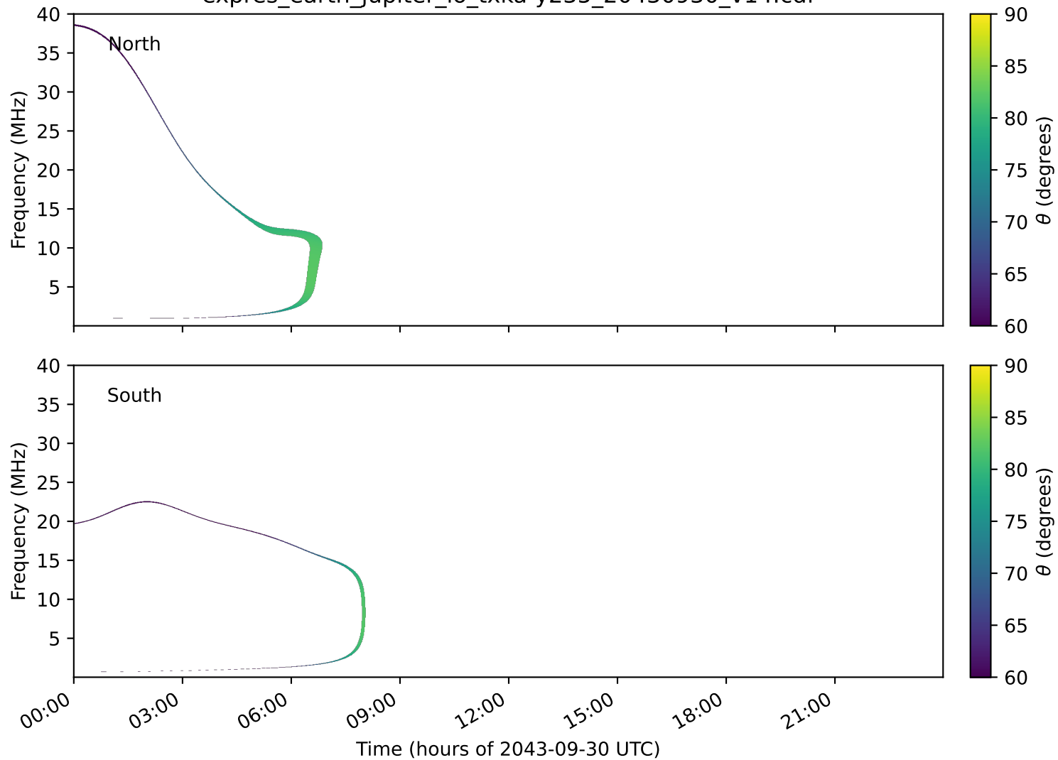
expres_earth_jupiter_io_txka-y235_20430930_v14.cdf
