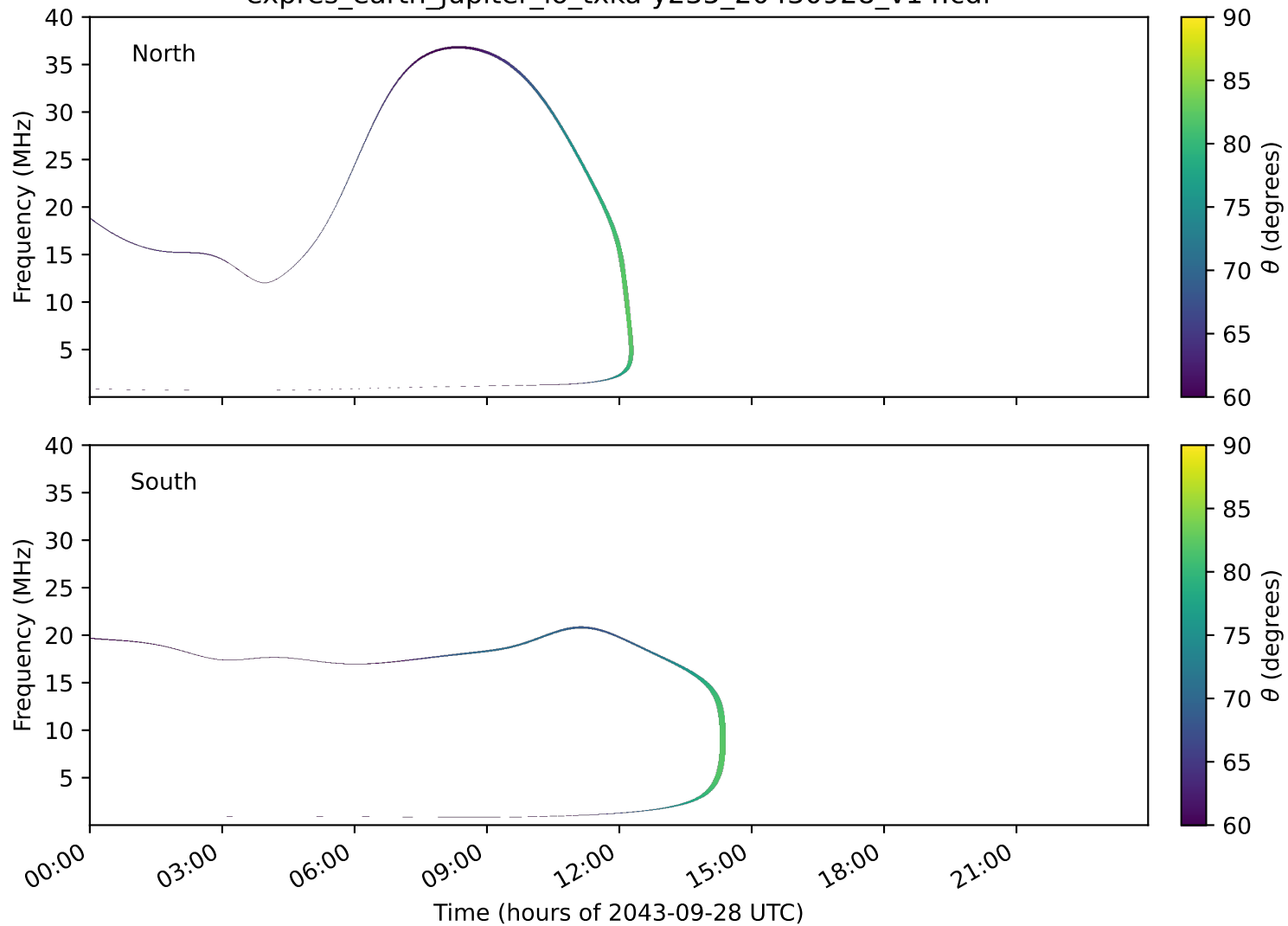
expres_earth_jupiter_io_txka-y235_20430928_v14.cdf
