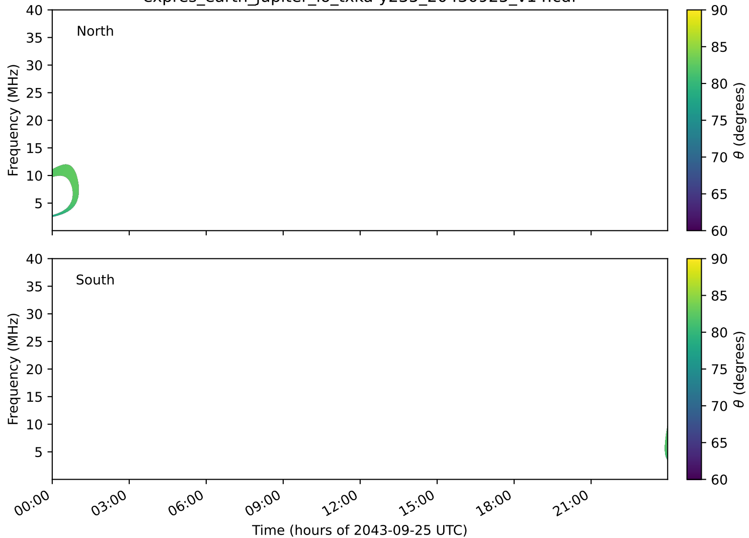
expres_earth_jupiter_io_txka-y235_20430925_v14.cdf
