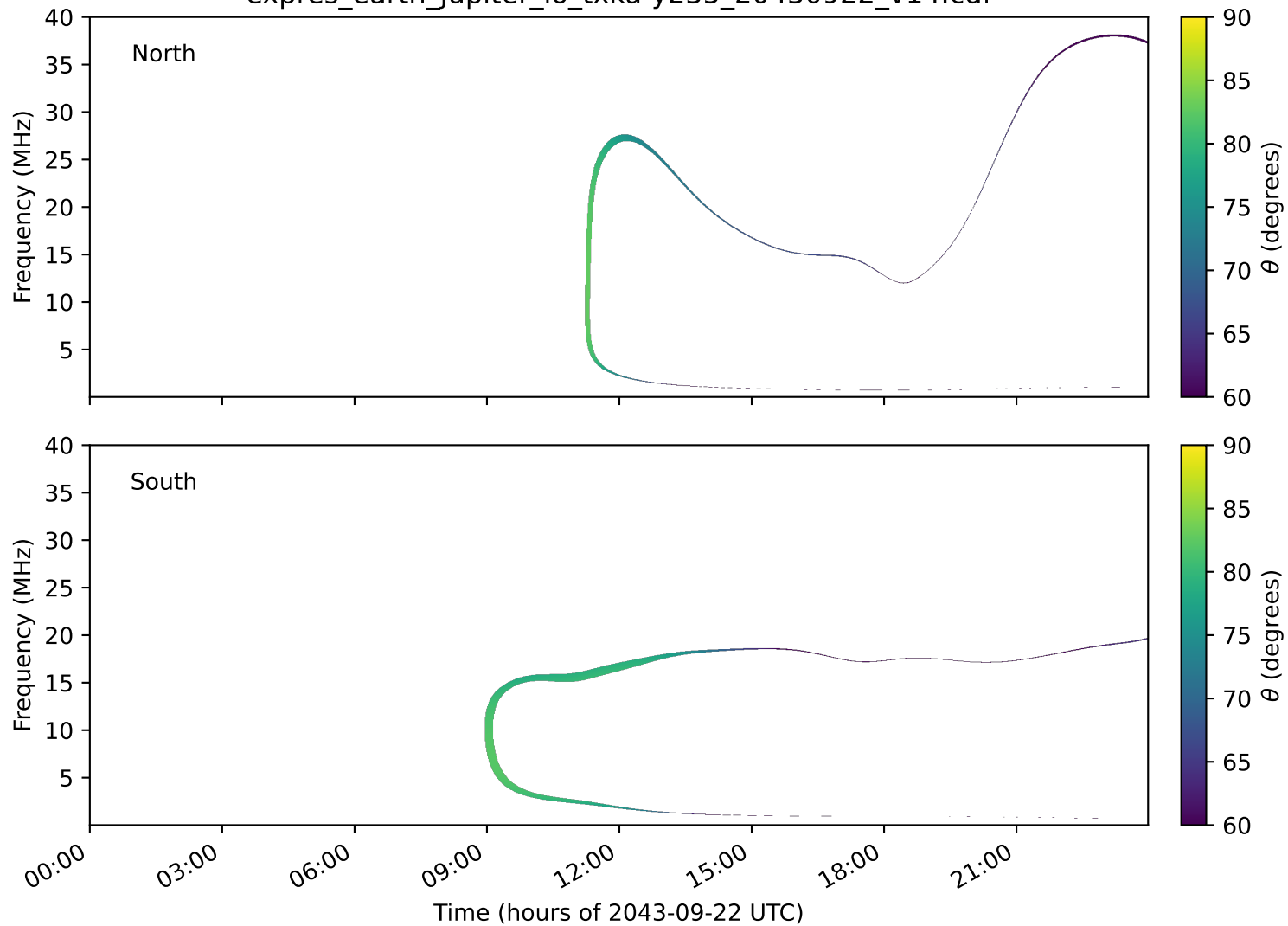
expres_earth_jupiter_io_txka-y235_20430922_v14.cdf
