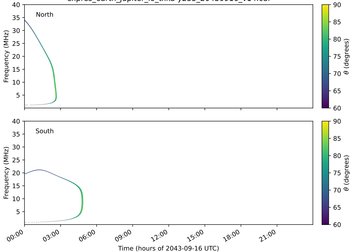
expres_earth_jupiter_io_txka-y235_20430916_v14.cdf
