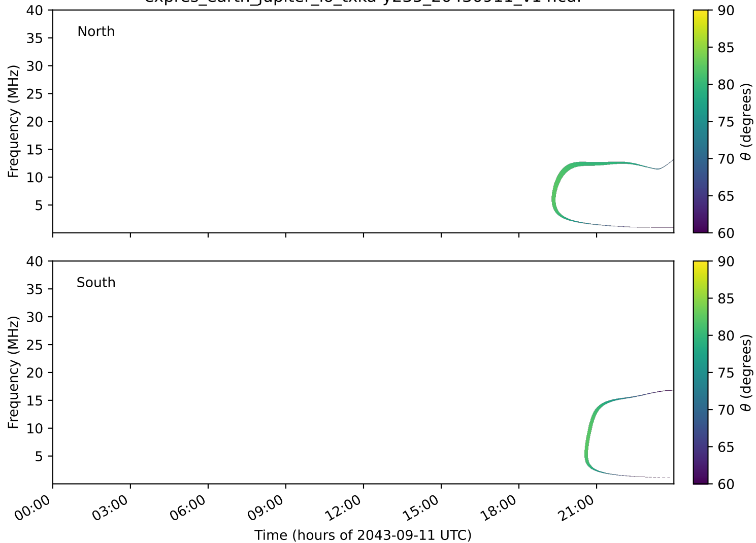
expres_earth_jupiter_io_txka-y235_20430911_v14.cdf
