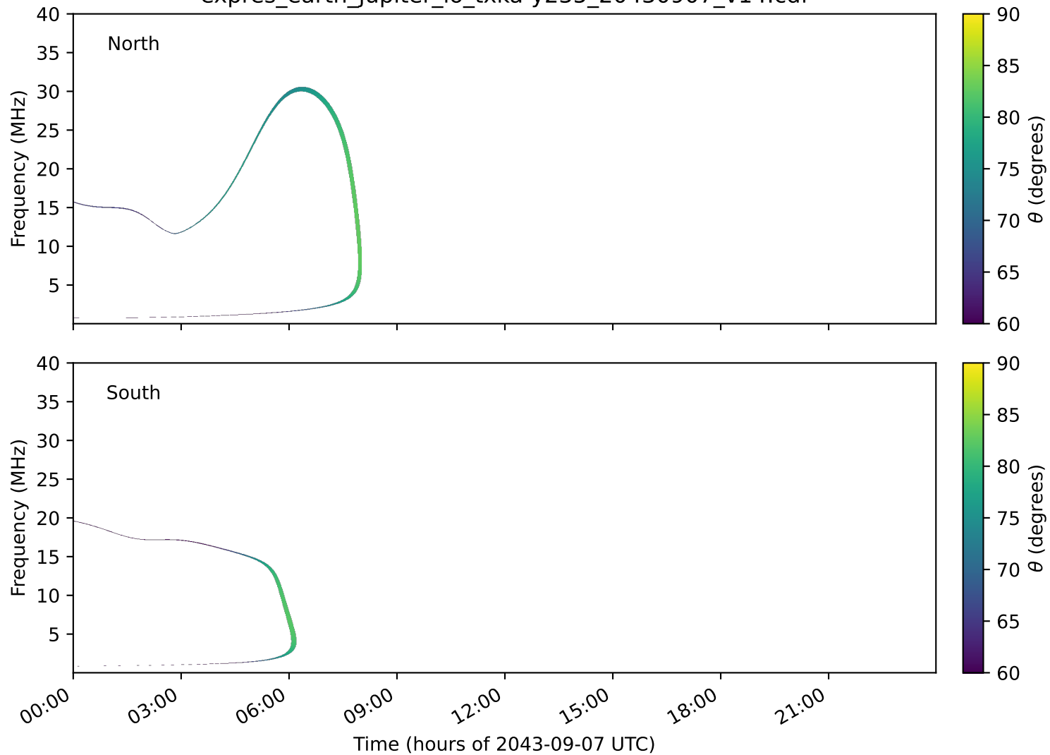
expres_earth_jupiter_io_txka-y235_20430907_v14.cdf
