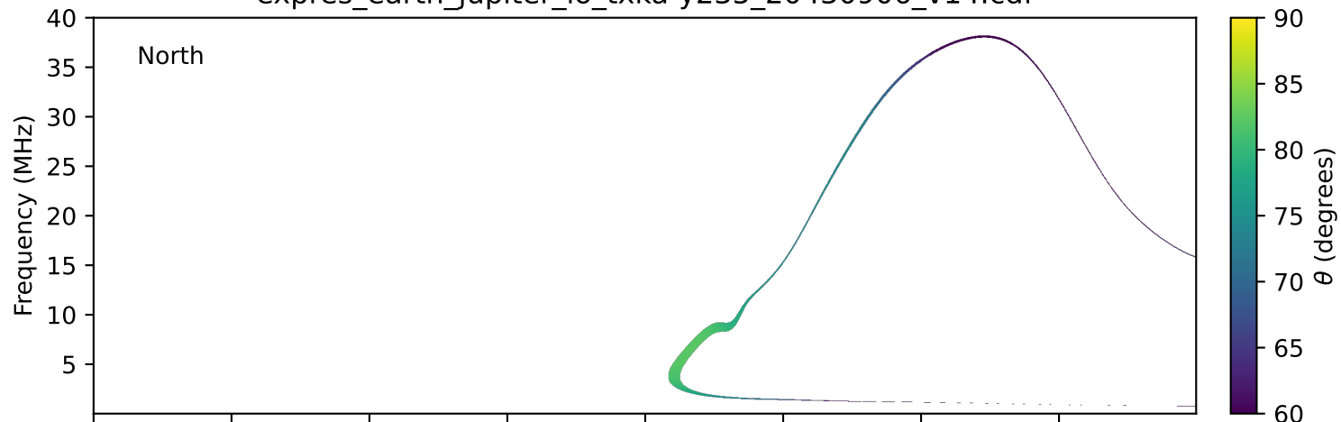
expres_earth_jupiter_io_txka-y235_20430906_v14.cdf
