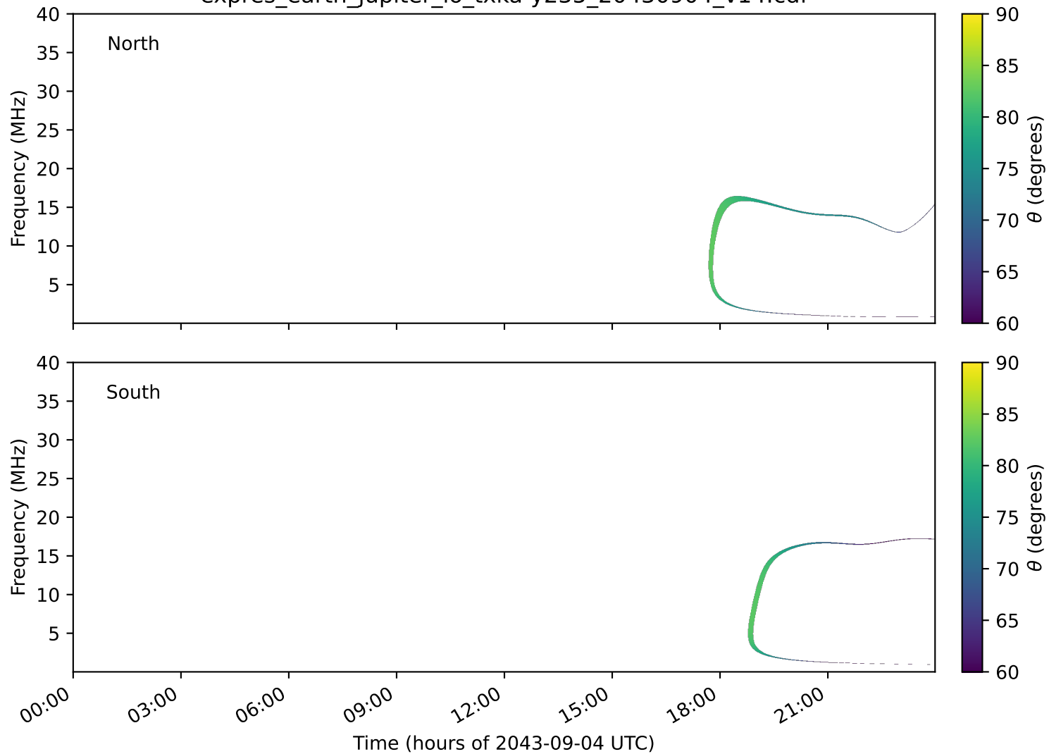
expres_earth_jupiter_io_txka-y235_20430904_v14.cdf
