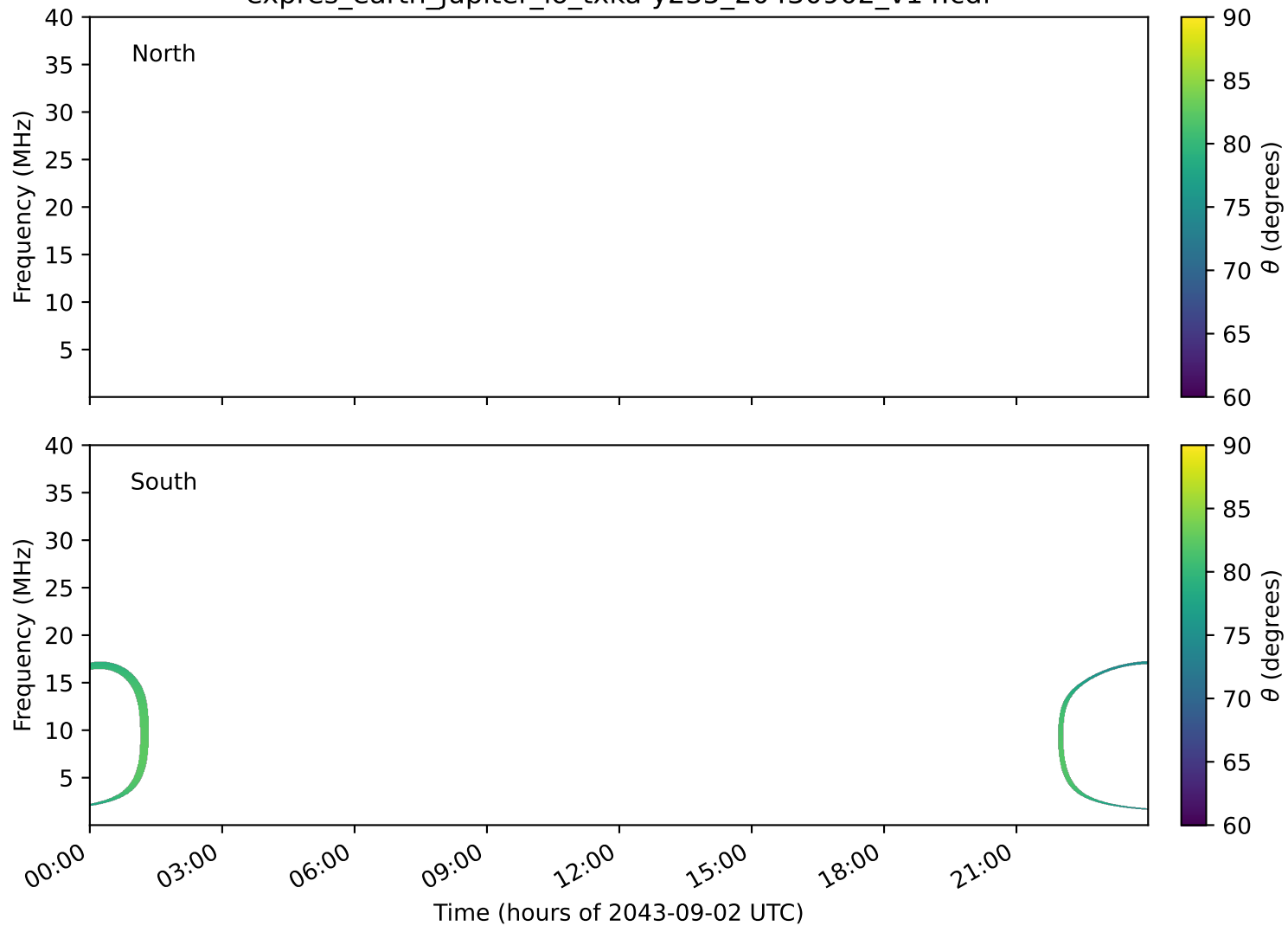
expres_earth_jupiter_io_txka-y235_20430902_v14.cdf
