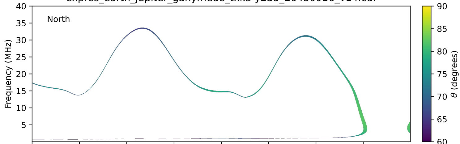
expres_earth_jupiter_ganymede_txka-y235_20430926_v14.cdf
