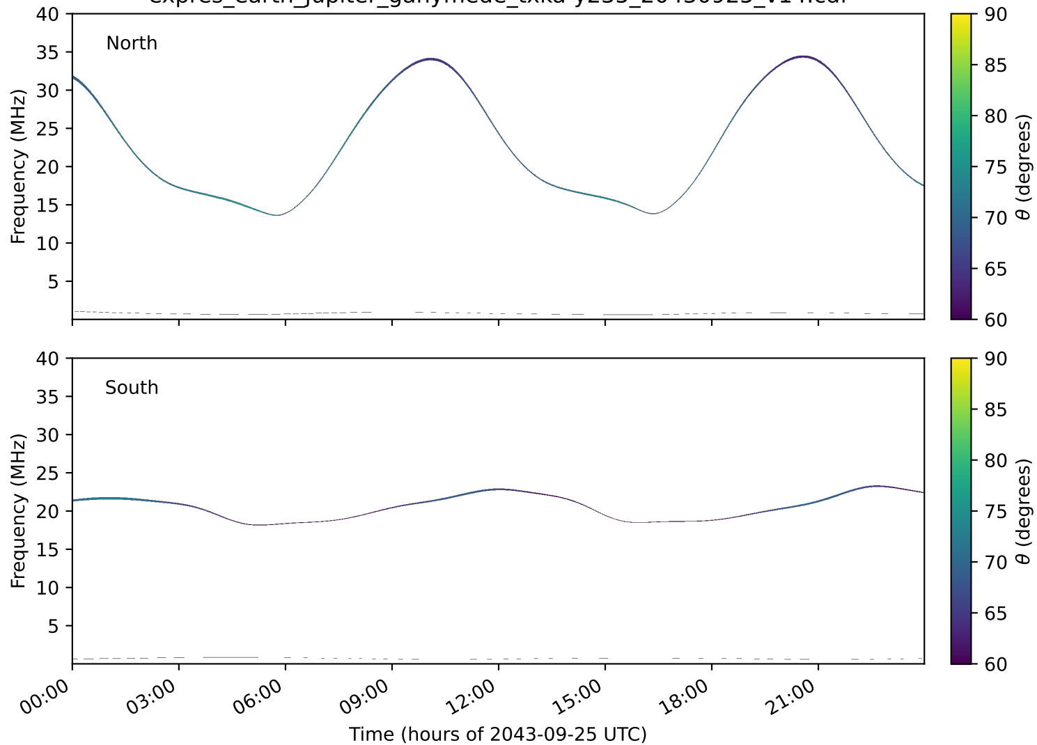
expres_earth_jupiter_ganymede_txka-y235_20430925_v14.cdf
