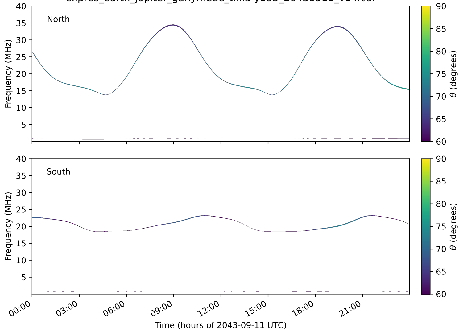
expres_earth_jupiter_ganymede_txka-y235_20430911_v14.cdf
