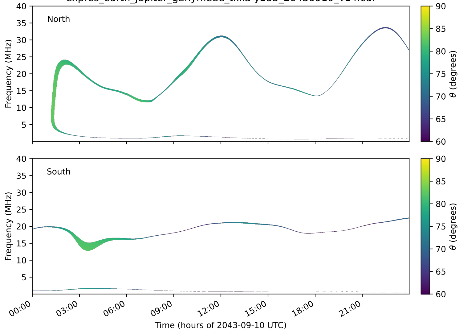
expres_earth_jupiter_ganymede_txka-y235_20430910_v14.cdf
