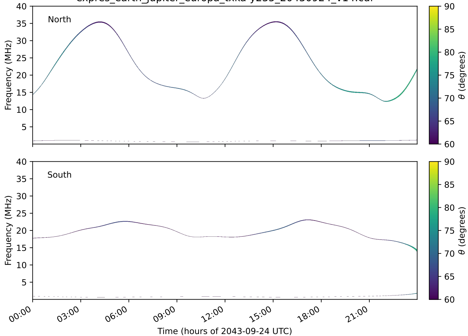
expres_earth_jupiter_europa_txka-y235_20430924_v14.cdf
