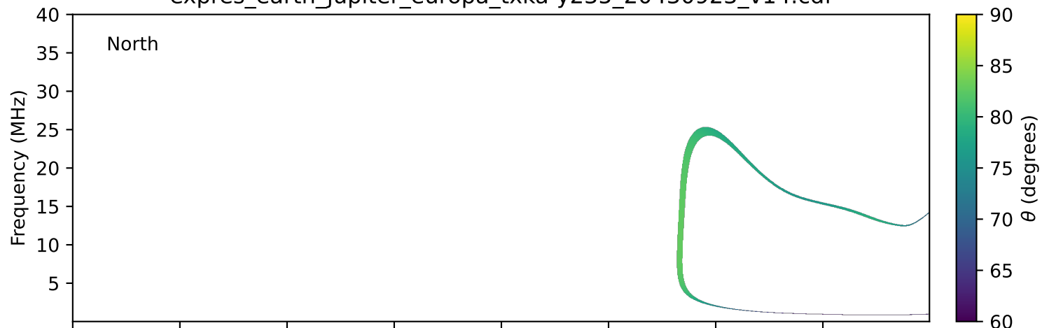
expres_earth_jupiter_europa_txka-y235_20430923_v14.cdf
