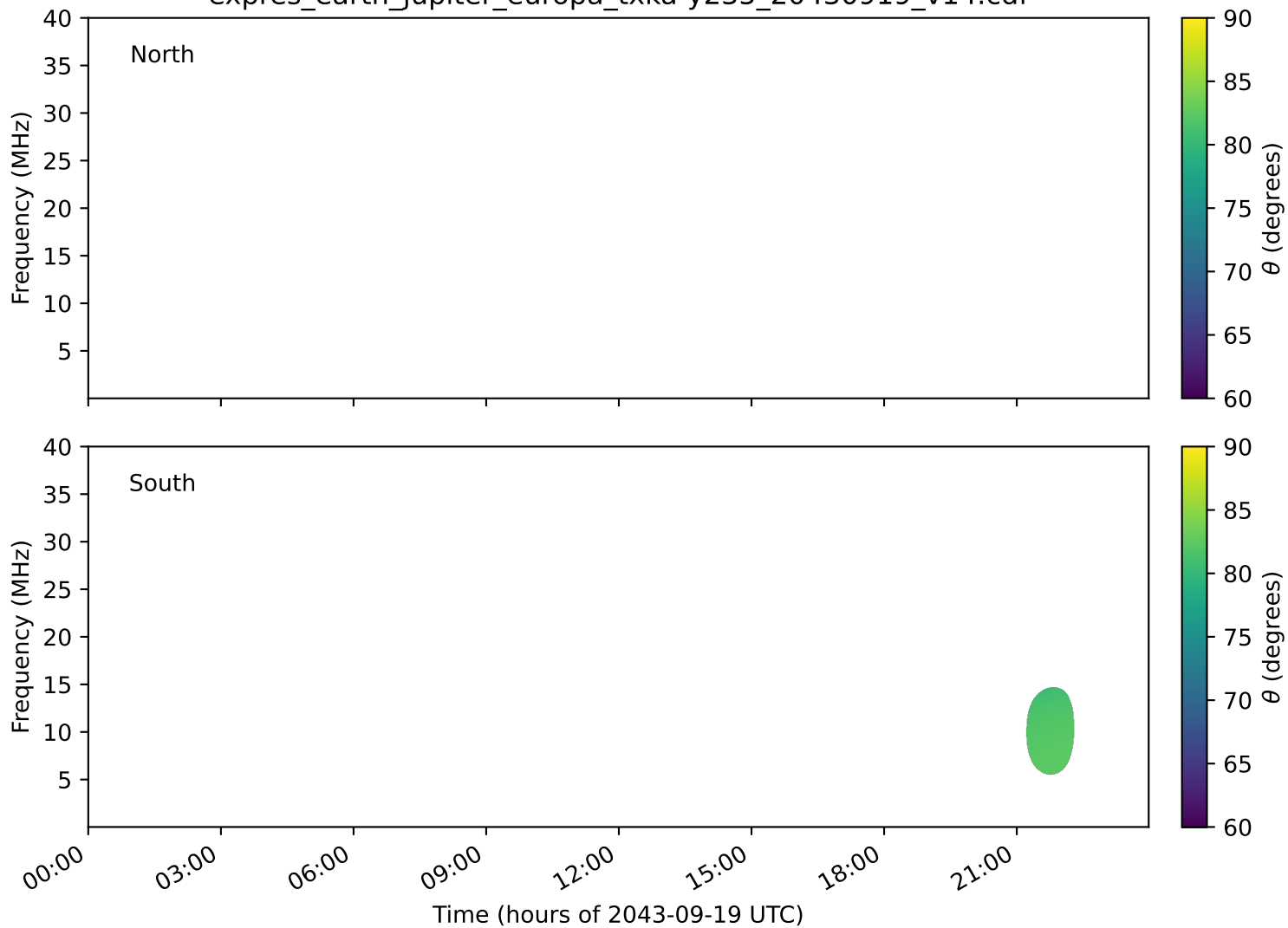
expres_earth_jupiter_europa_txka-y235_20430919_v14.cdf
