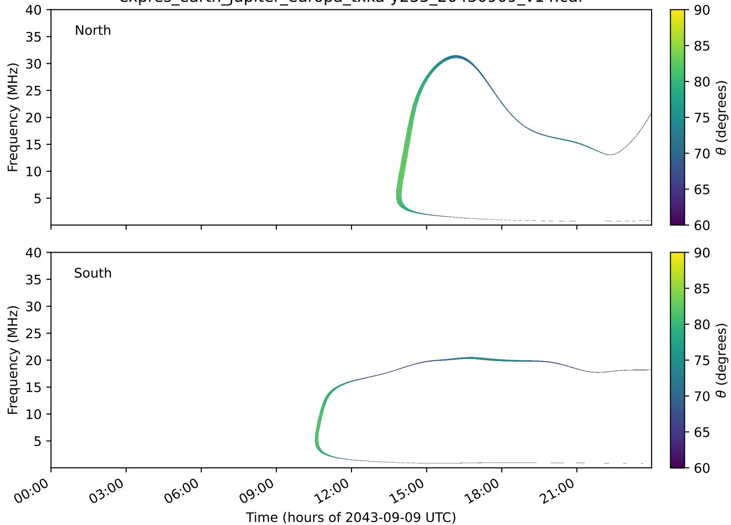
expres_earth_jupiter_europa_txka-y235_20430909_v14.cdf
