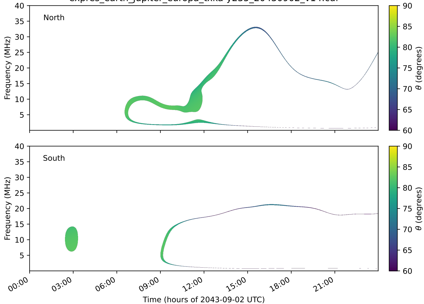
expres_earth_jupiter_europa_txka-y235_20430902_v14.cdf
