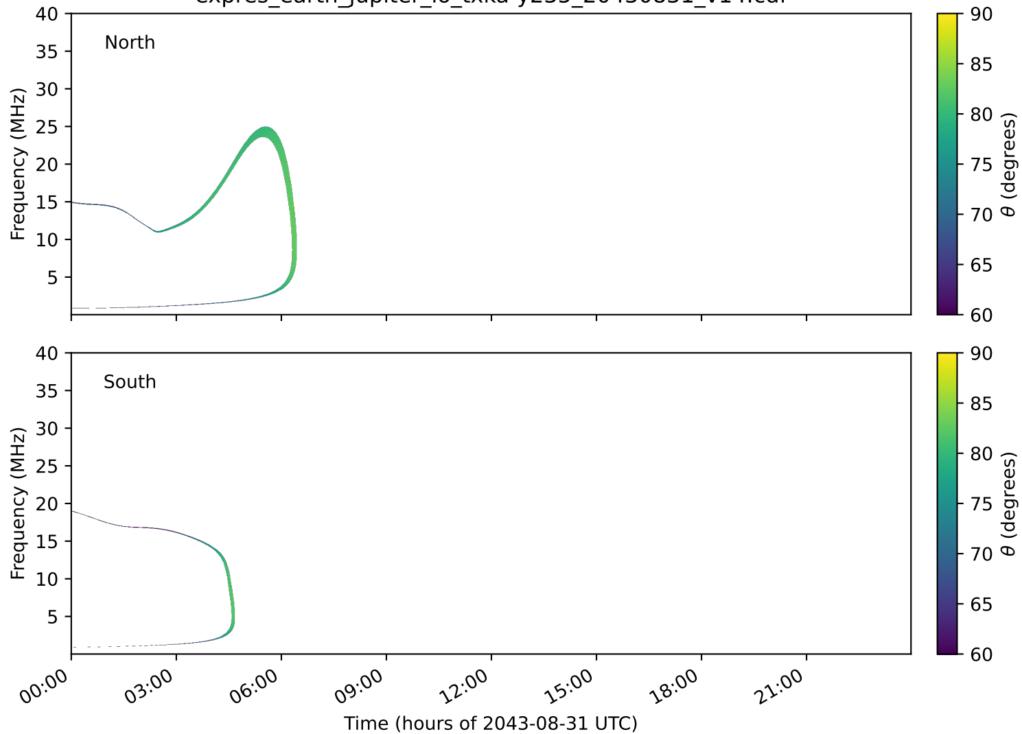
expres_earth_jupiter_io_txka-y235_20430831_v14.cdf
