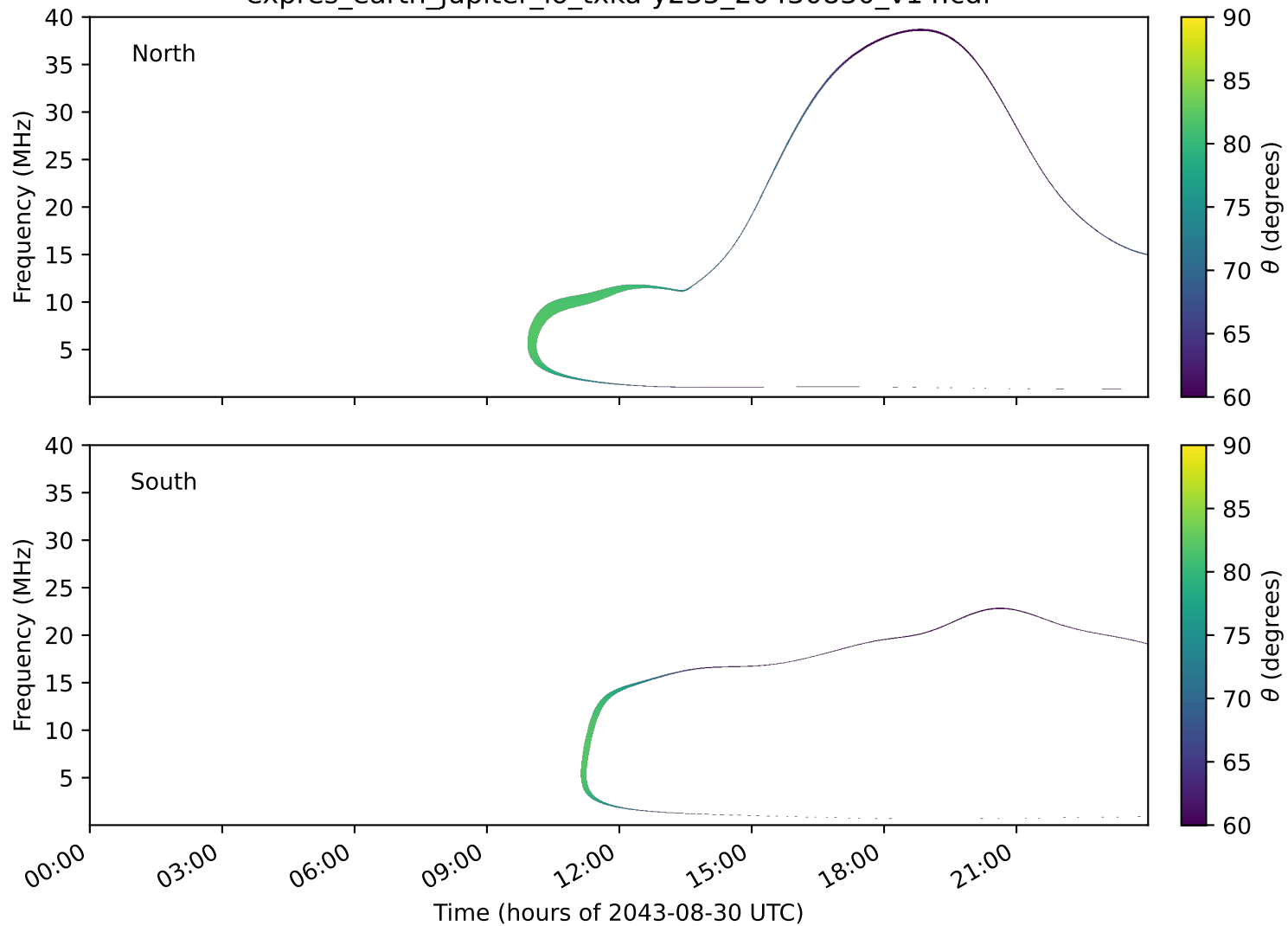
expres_earth_jupiter_io_txka-y235_20430830_v14.cdf
