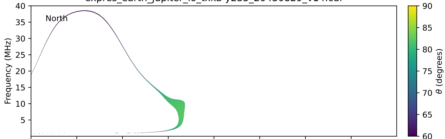
expres_earth_jupiter_io_txka-y235_20430829_v14.cdf
