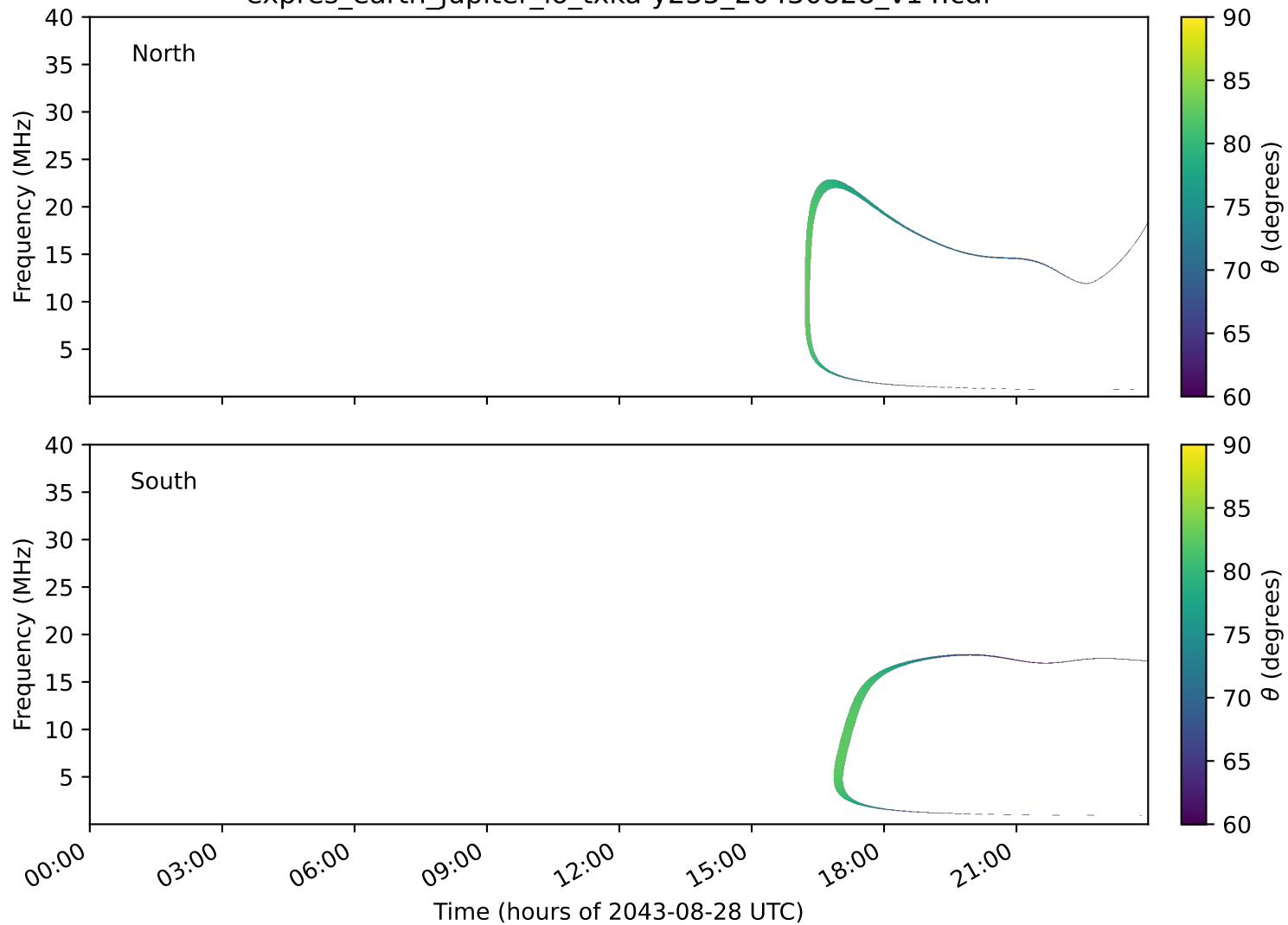
expres_earth_jupiter_io_txka-y235_20430828_v14.cdf
