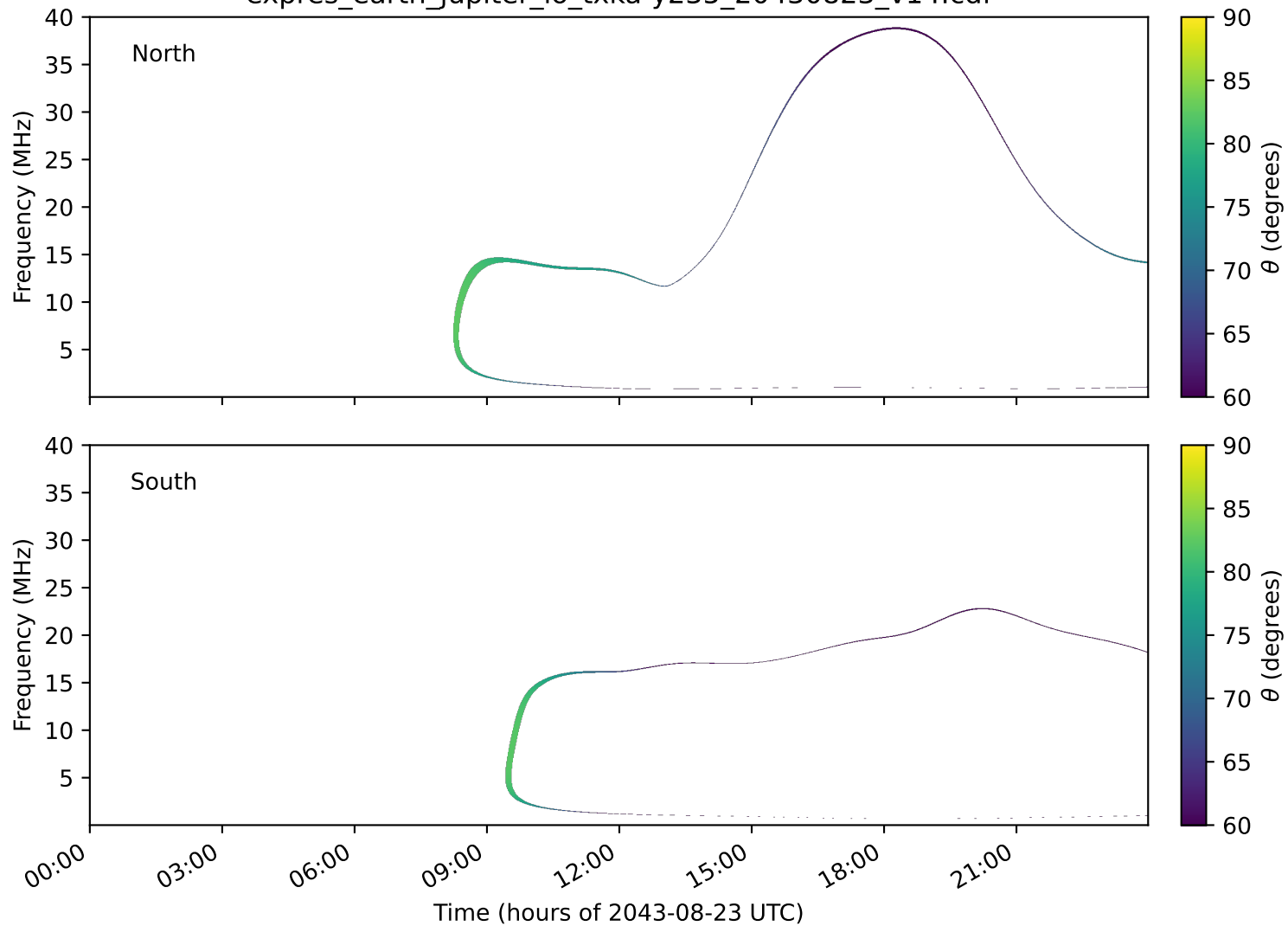
expres_earth_jupiter_io_txka-y235_20430823_v14.cdf
