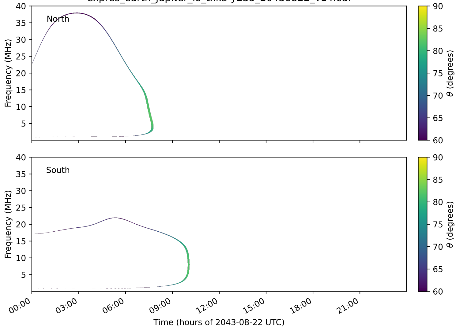
expres_earth_jupiter_io_txka-y235_20430822_v14.cdf
