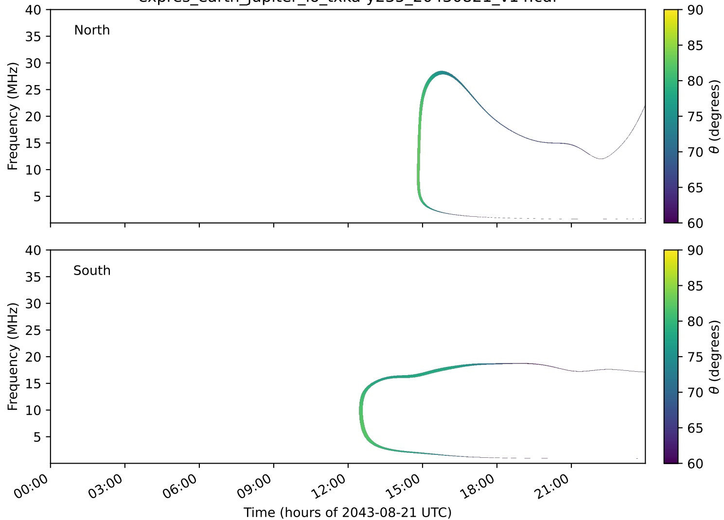
expres_earth_jupiter_io_txka-y235_20430821_v14.cdf
