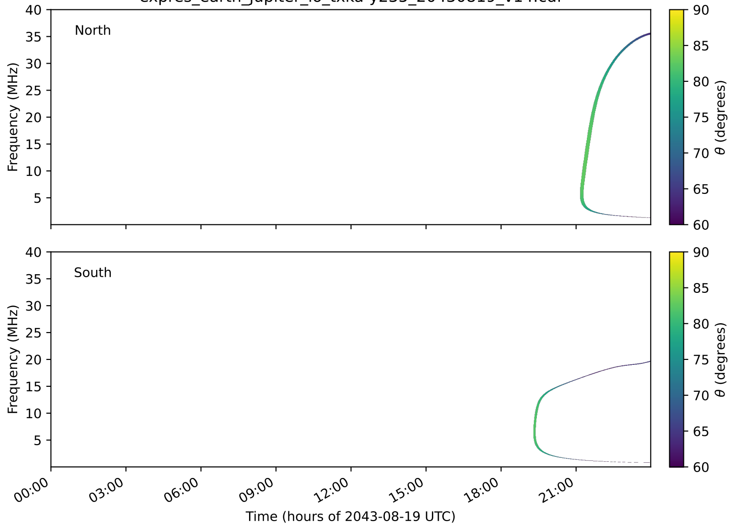
expres_earth_jupiter_io_txka-y235_20430819_v14.cdf
