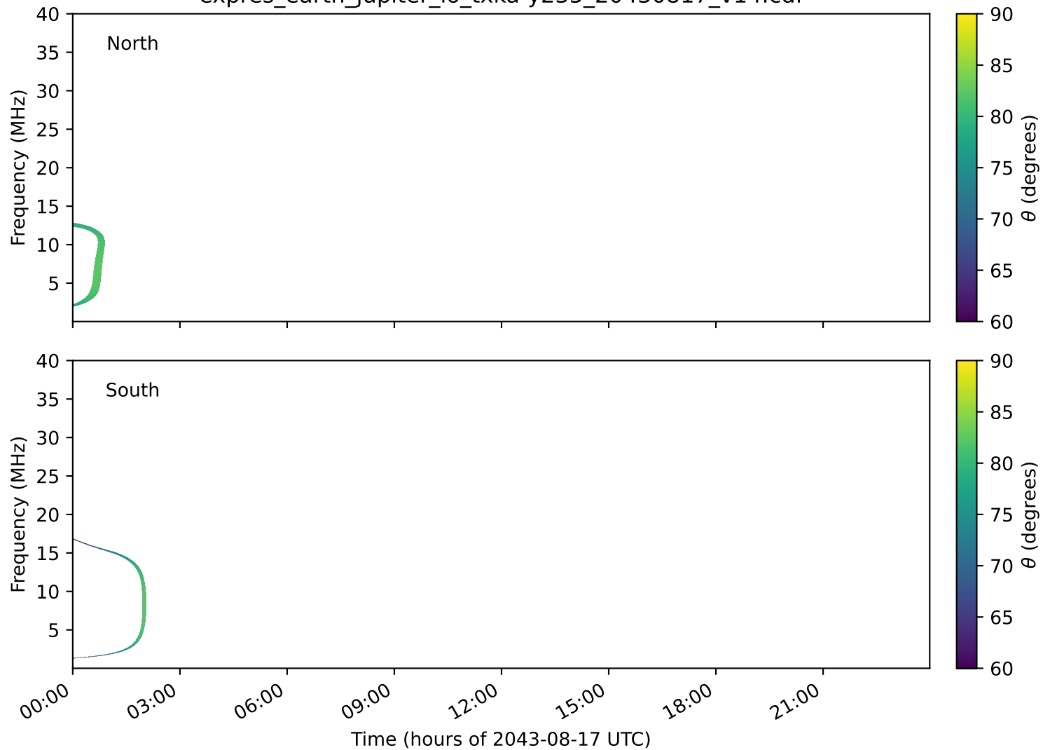
expres_earth_jupiter_io_txka-y235_20430817_v14.cdf
