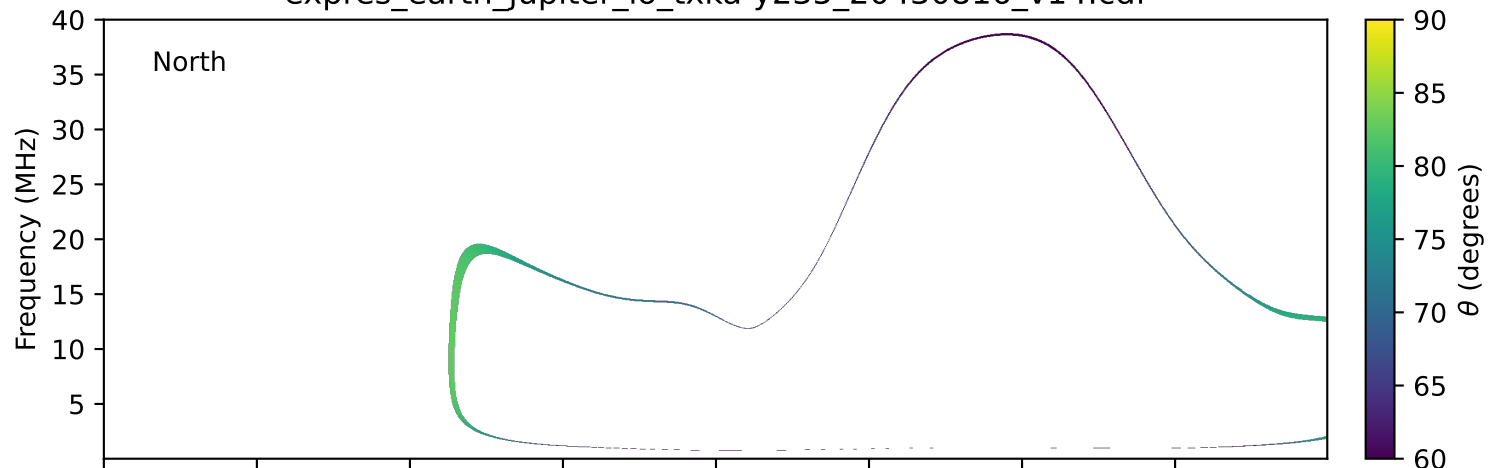
expres_earth_jupiter_io_txka-y235_20430816_v14.cdf
