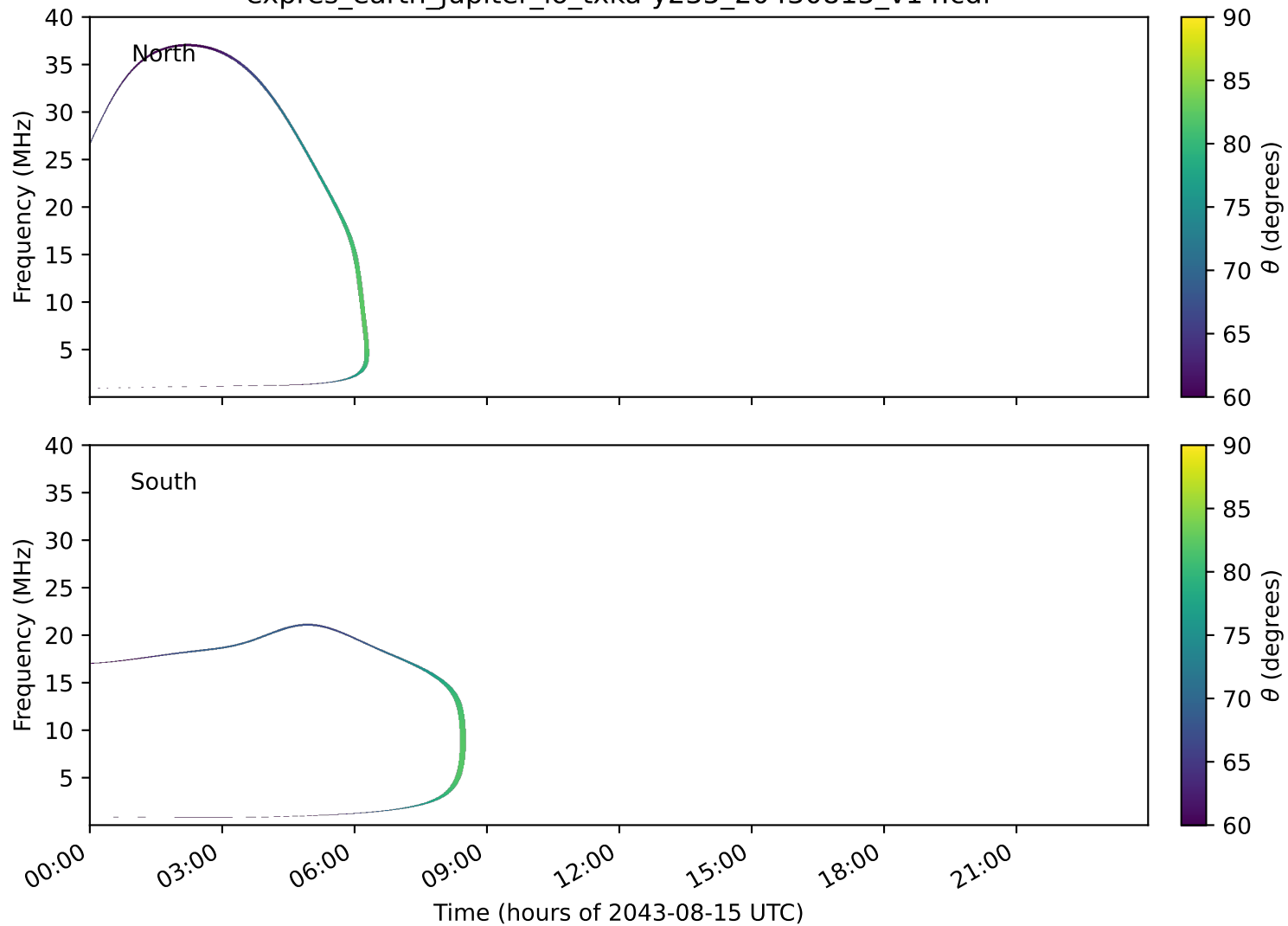
expres_earth_jupiter_io_txka-y235_20430815_v14.cdf
